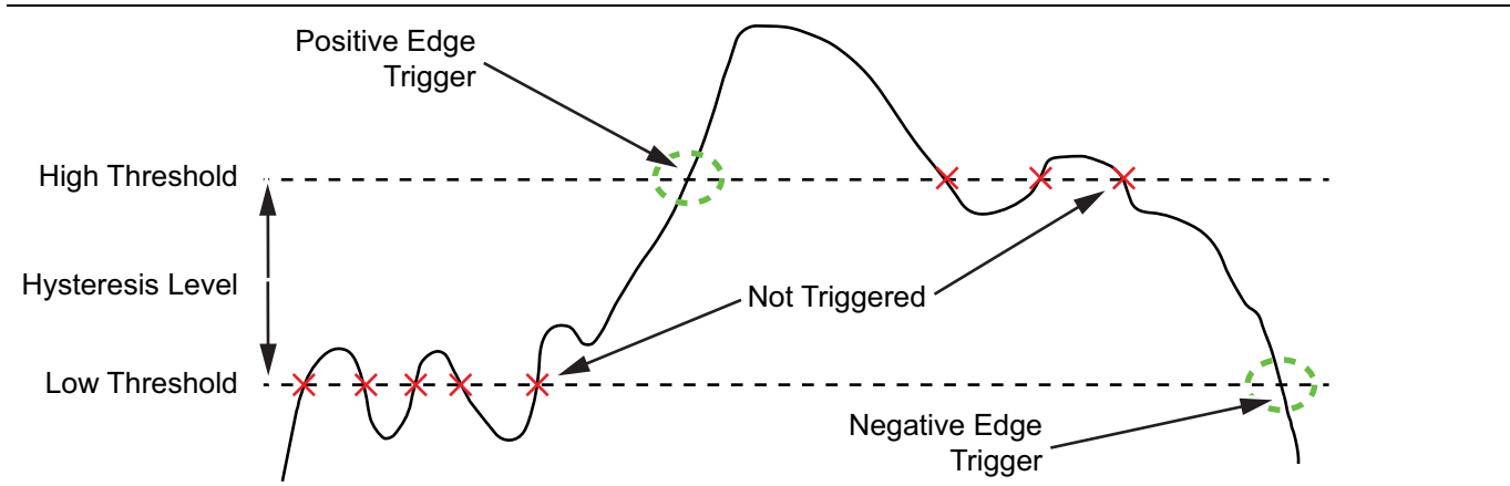
Figure 4-31. Trigger Levels and Hysteresis
