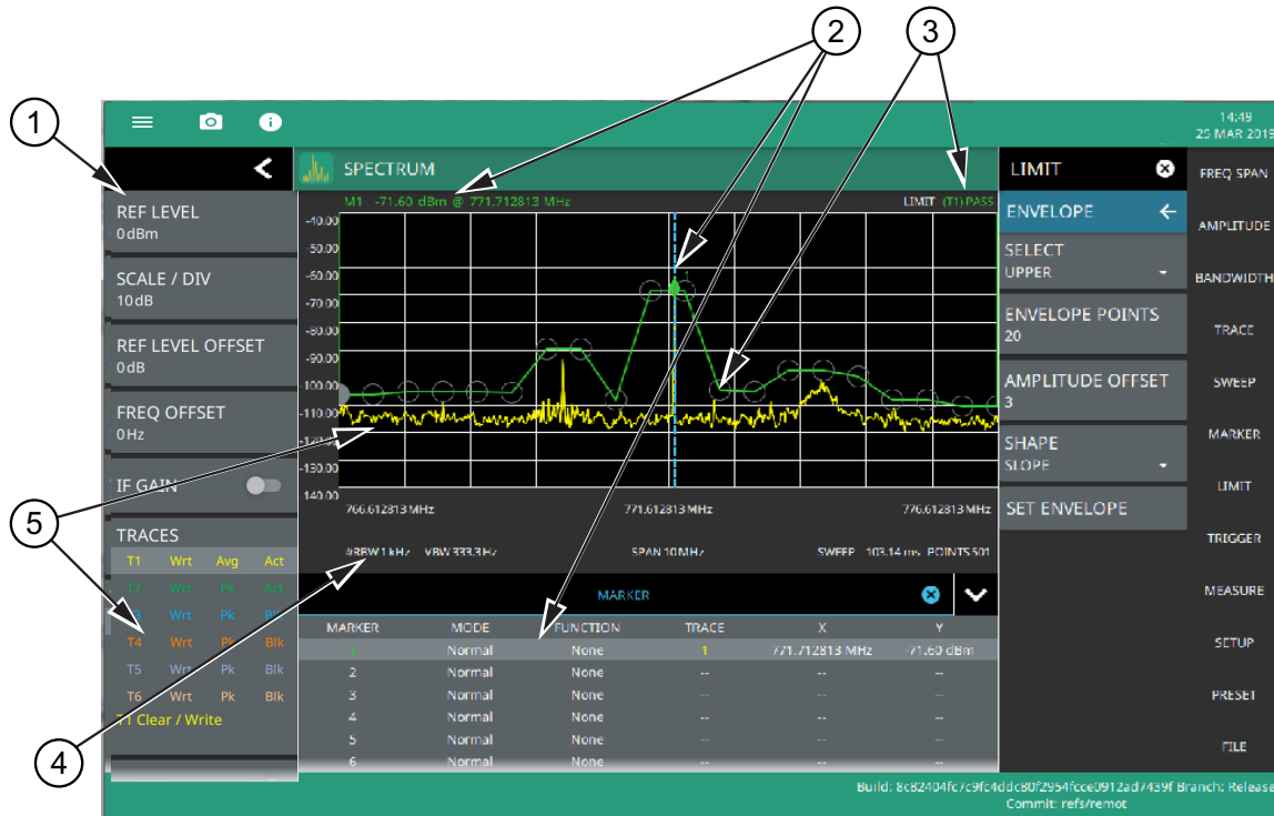
Figure 4-1. Spectrum Analyzer: Spectrum View (1 of 2)
